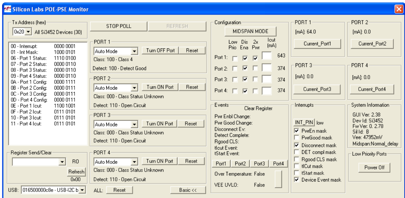
Figure 12. Result of Putting Port 1 into Auto and POE+ Mode and Plugging in the Si3401 Class 4 PD with a 10 \Omega Load
